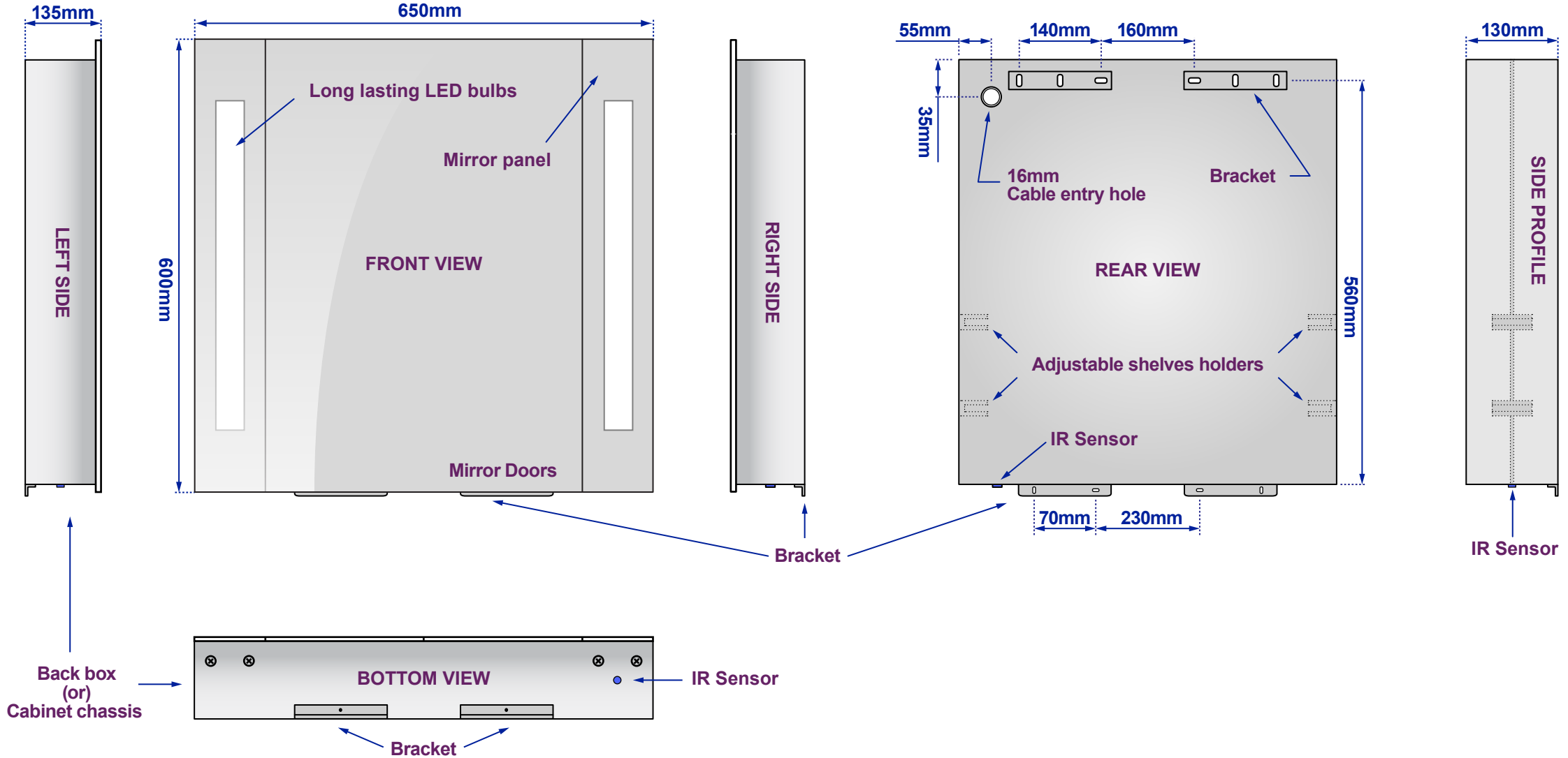
Views of complete assembly - With Mirror Door(s)/Panel(s)
