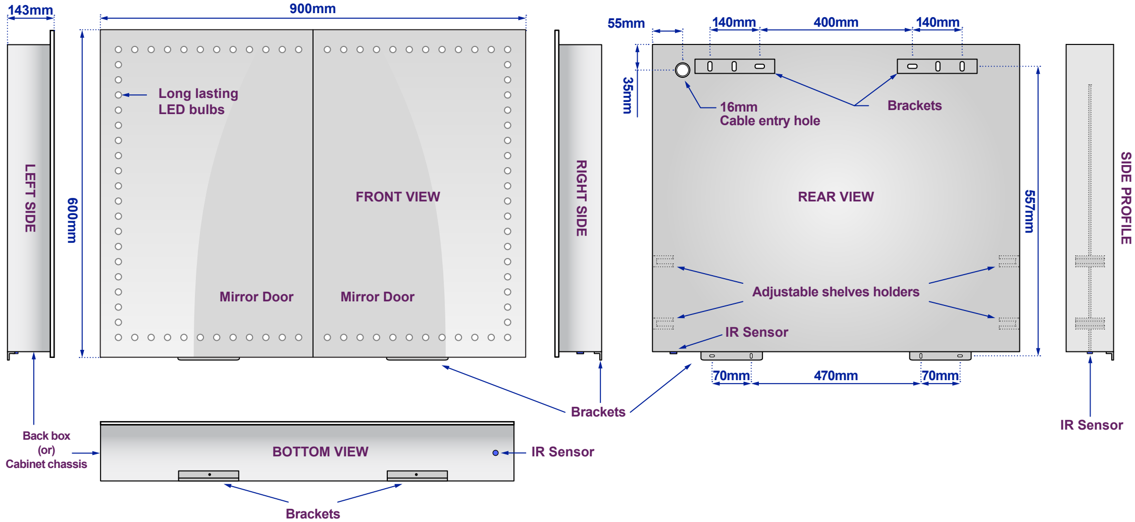
Views of complete assembly - With Mirror Door(s)/Panel(s)
