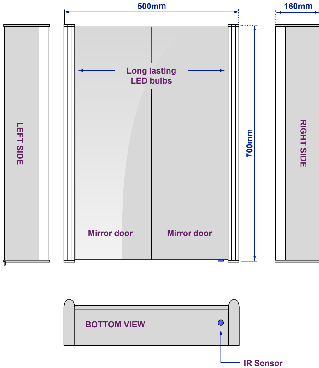
Views of complete assembly
